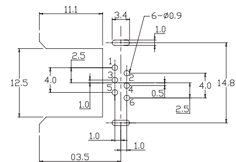
COMPONENT SIDE PCB LAYOUT
